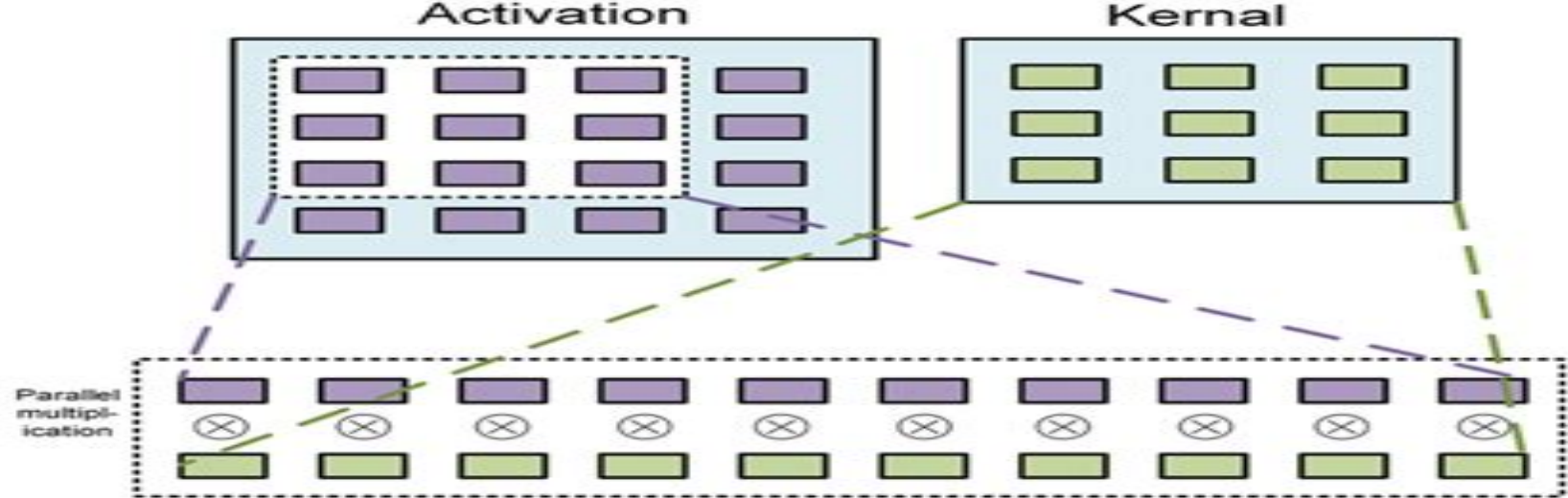
(a) Parallel architecture based on a fixed convolution window in non-sparsity-aware works
