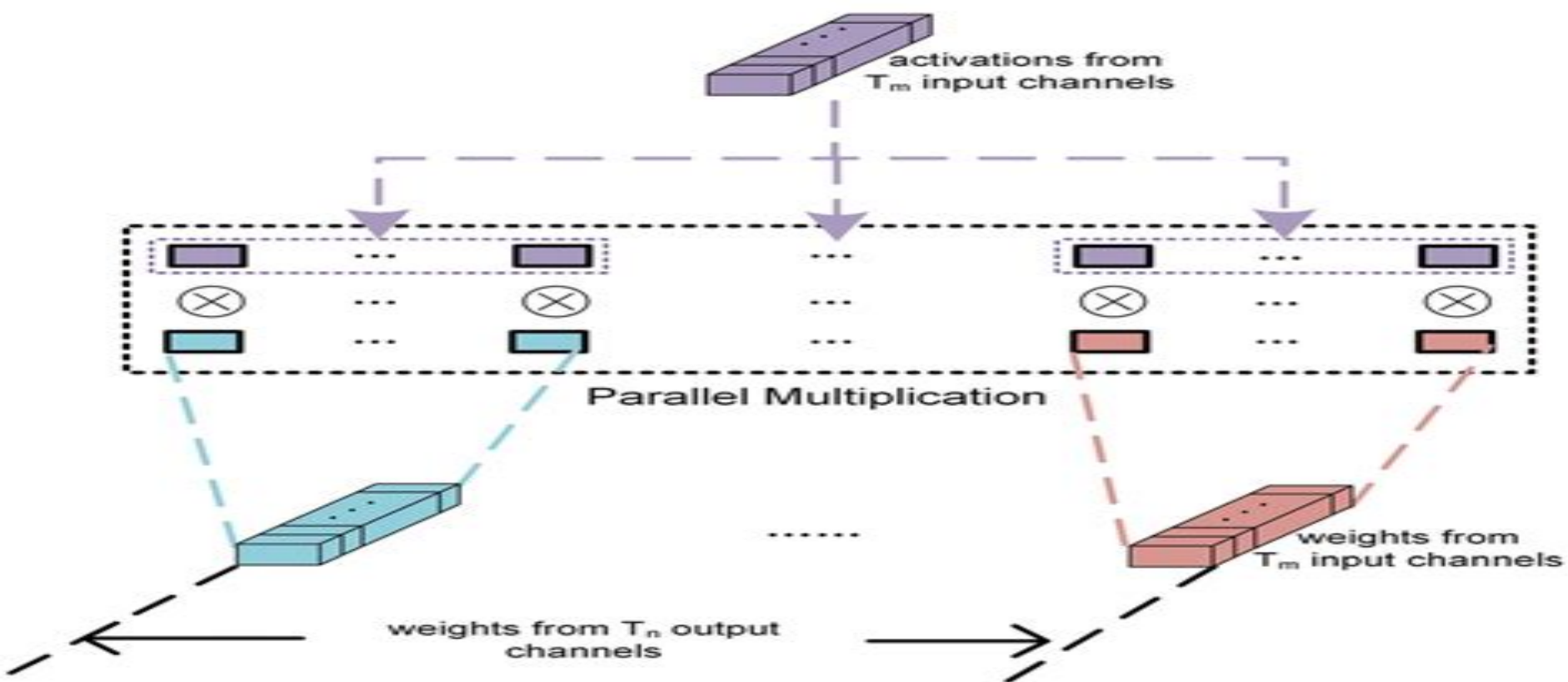
(b) Parallel architecture based on input and output channels in sparse network
