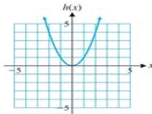
(B) Square function h(x) = x^2 Domain: \mathcal{R} Range: [0, \infty)
