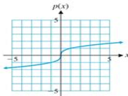
(E) Cube root function p(x) = \sqrt[3]{x} Domain: \mathcal{R} Range: \mathcal{R}
