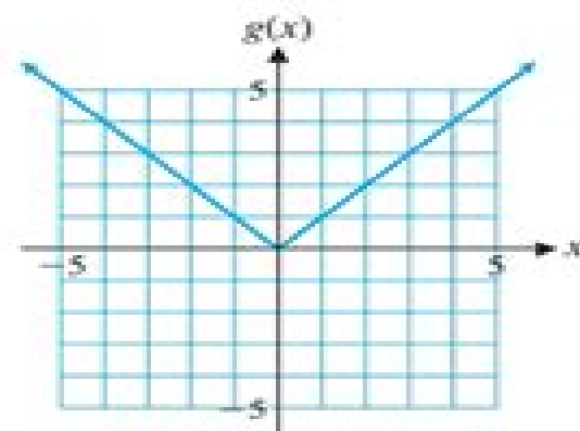
(F) Absolute value function g(x) = |x| Domain: \mathcal{R} Range: [0, \infty)
