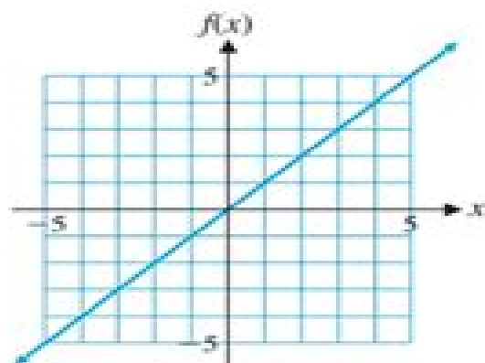
(A) Identity function f(x) = x Domain: \mathcal{R} Range: \mathcal{R}
