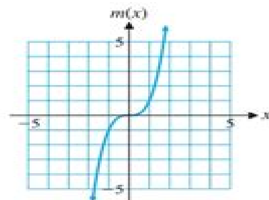
(C) Cube function m(x) = x^3 Domain: \mathcal{R} Range: \mathcal{R}
