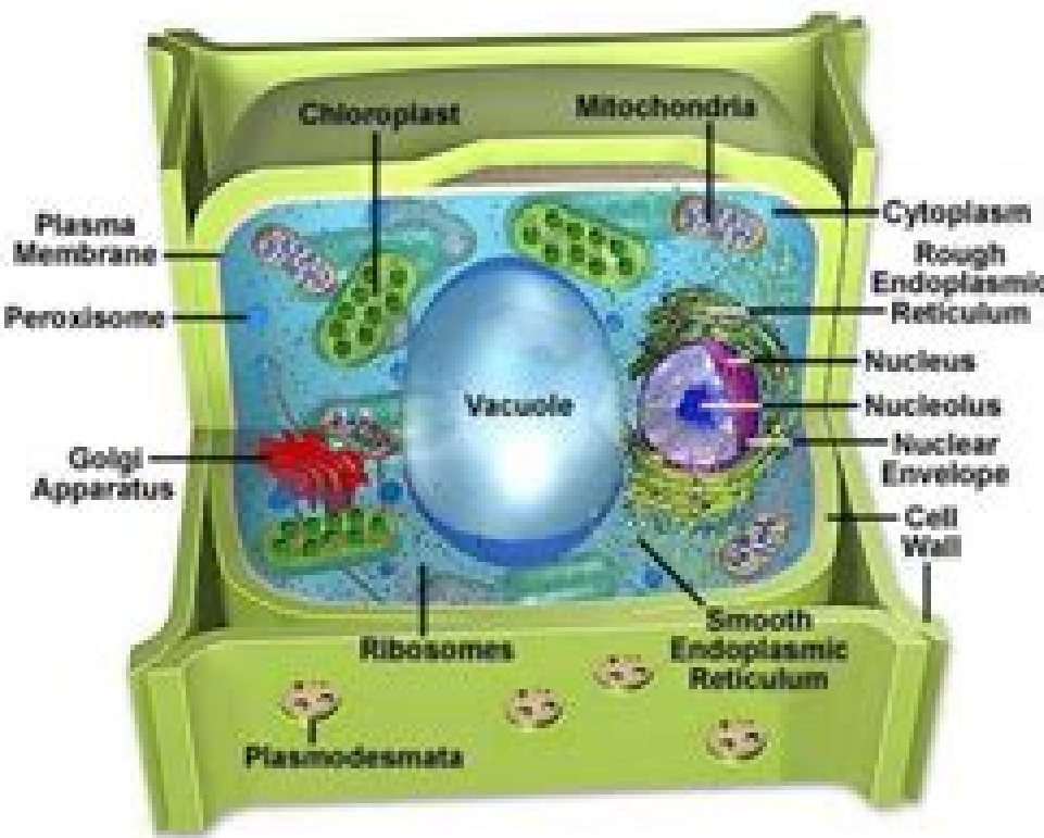
PLANT CELL
