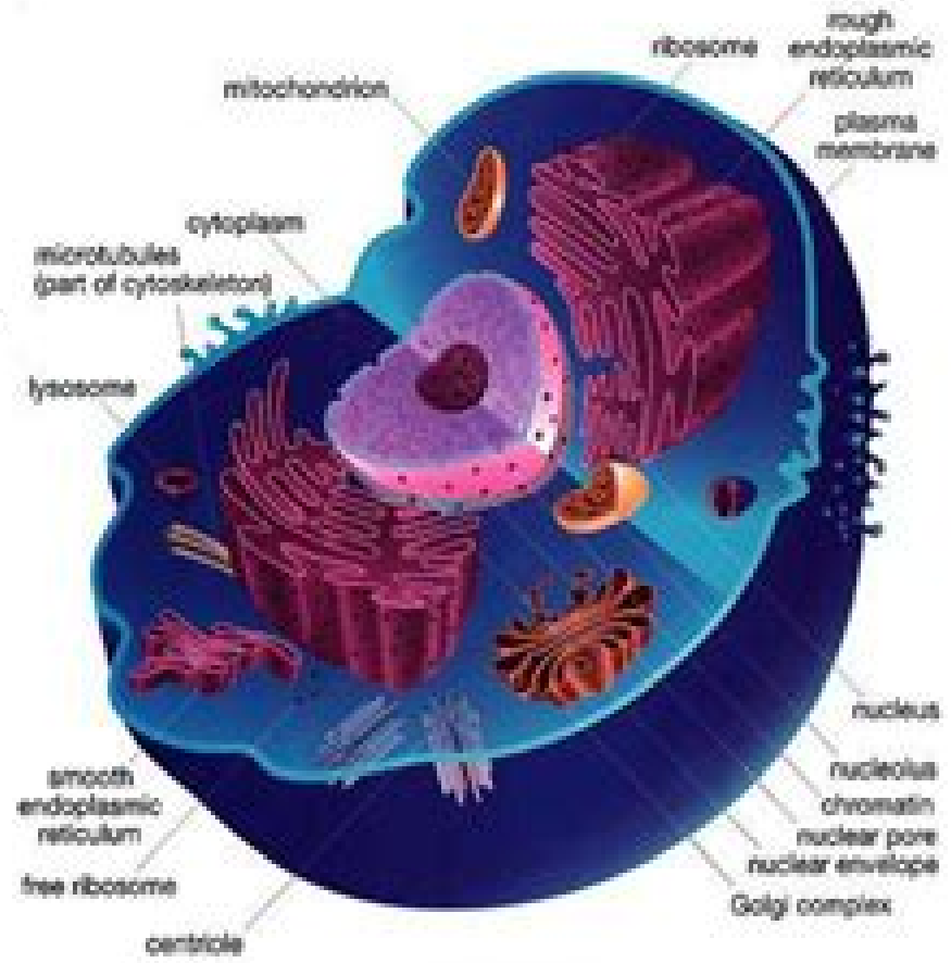
ANIMAL CELL
