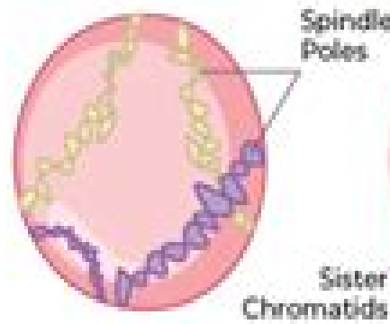
Early Prophase
