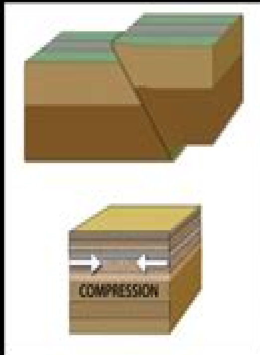
Reverse fault
