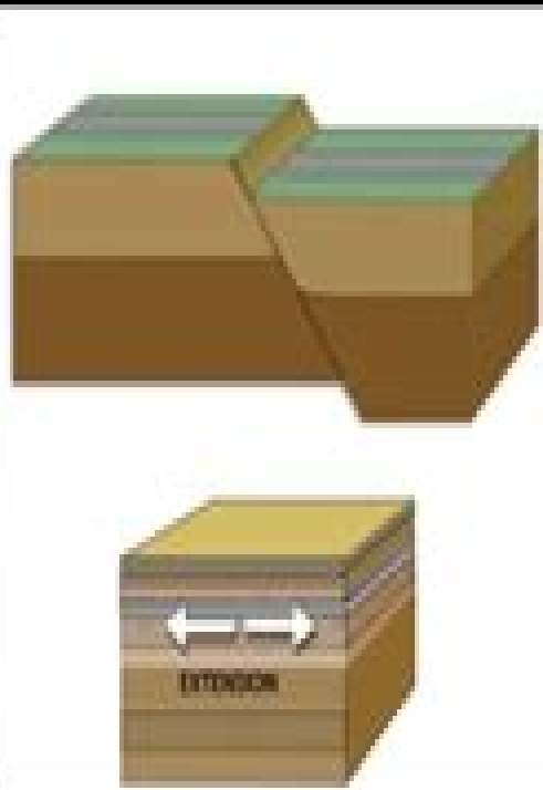
Normal fault
