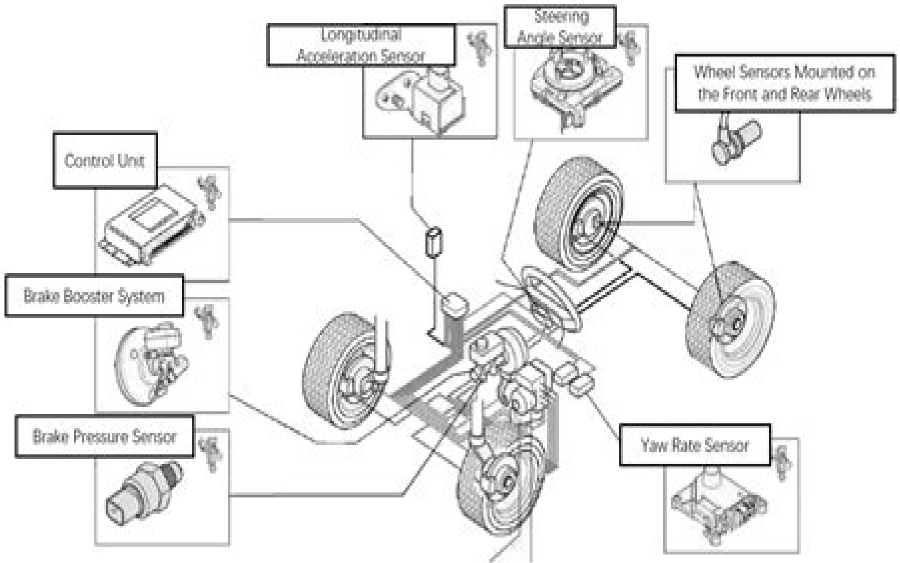
Structure and Components of the ESP System
