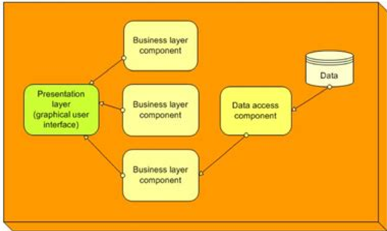
Figure 10-1 Component-based development
