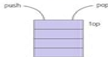
Stack
