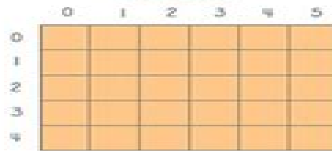
Matrix
