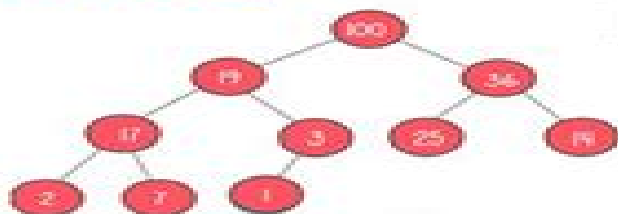
Max Heap
