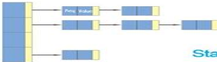
HashMap
