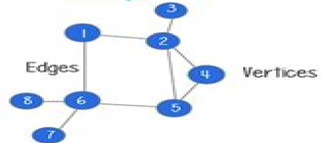
Graph
