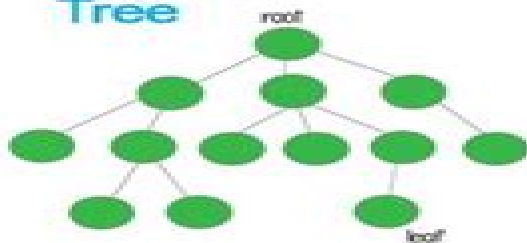
Tree
