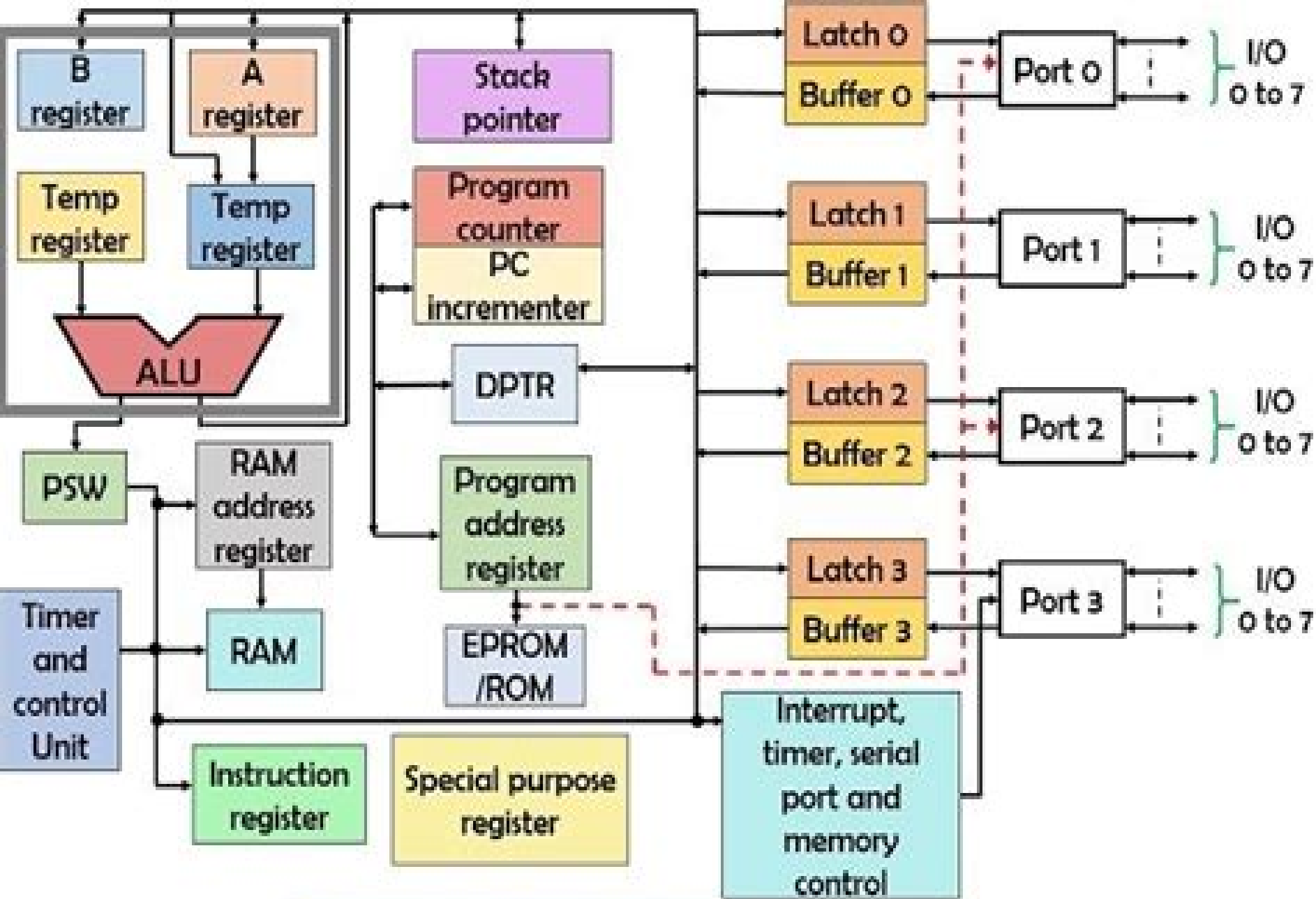
Architecture of 8051 Microcontroller
