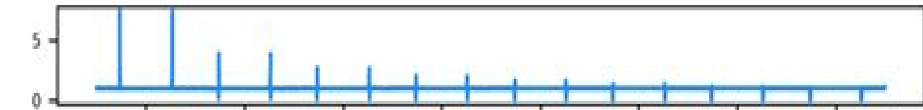
Residuals
