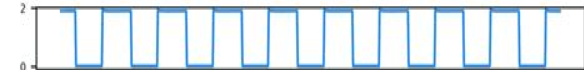
Seasonality
